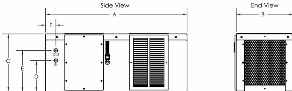
Wine Guardian water-cooled unit with ductable supply and return evaporator section.
